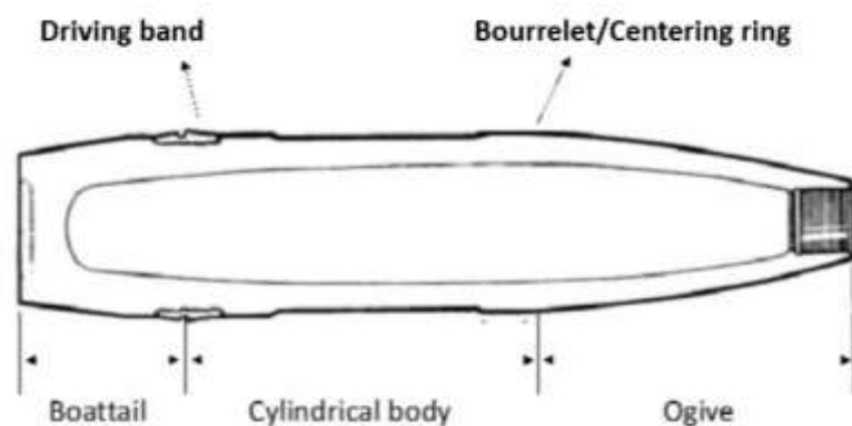
FIGURE 11: GENERIC ARTILLERY SHELL DESIGN
